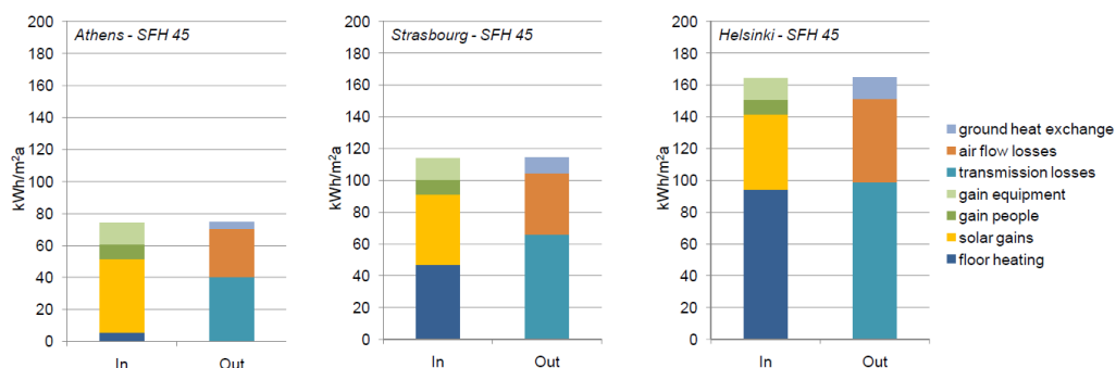
Figure 7: Building energy balances of a Single Family building with an annual heating demand of 45 kWh/(m 2 year) - SFH 45 - at three different locations.
